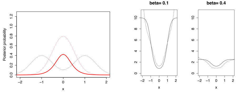
(a) Class conditional distributions (thin lines) and the posterior distribution of the minority class (thicker line). (b) \frac{dp_s}{dp} (solid lines), \sqrt{\frac{p_s}{\nu}} (dotted lines).
